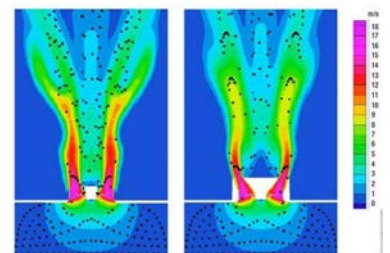
No Axitop Axitop Energy efficiency improved by Axitop
