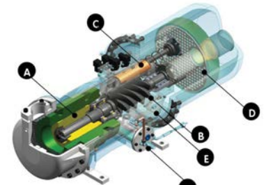
A Electric motor B Twin screw rotor C Continuous capacity control D Oil separator E Economiser door F Oil level sensor control
